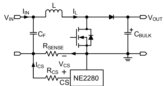
Figure 6 Current Sensing
