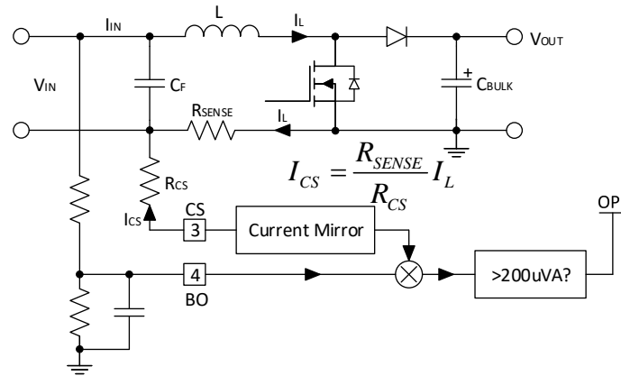
Figure 15 Over-Power Limitation
