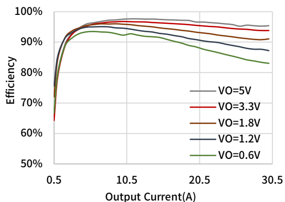
图 13-1 Efficiency 12V Input
