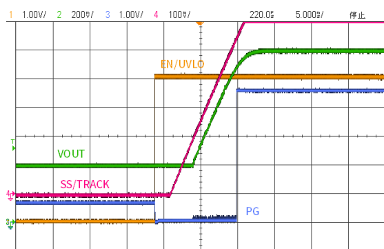
图 13-5 Pre-bias Start
